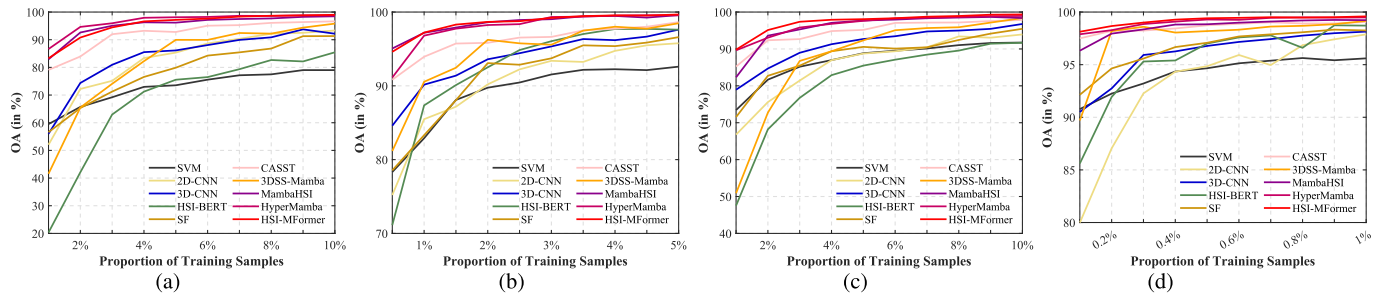
Fig. 13. Classification performance of the compared methods with different proportions of labeled data on four datasets. (a) Indian Pines. (b) Pavia University. (c) Houston 2013. (d) WHU-Hi-LongKou.
