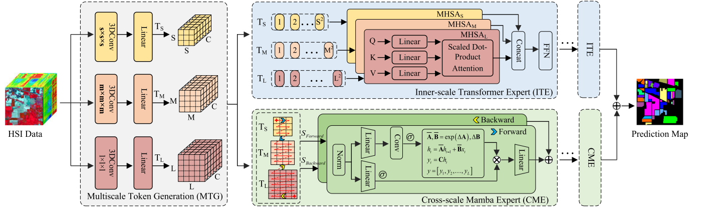
Fig. 3. Overall architecture of the hybrid Mamba-Transformer framework (HSI-MFormer), taking the parallel structure as an example.
