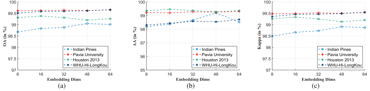
Fig. 11. Sensitivity analysis for the proposed method with different feature embedding dimensions in terms of (a) OA, (b) AA, and (c) Kappa.
