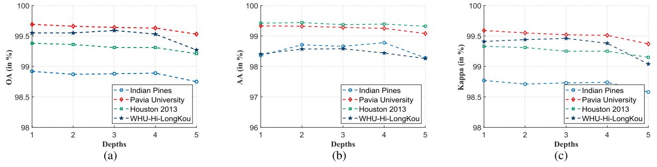
Fig. 10. Sensitivity analysis for the proposed method with different stage depths in terms of (a) OA, (b) AA, and (c) Kappa.
