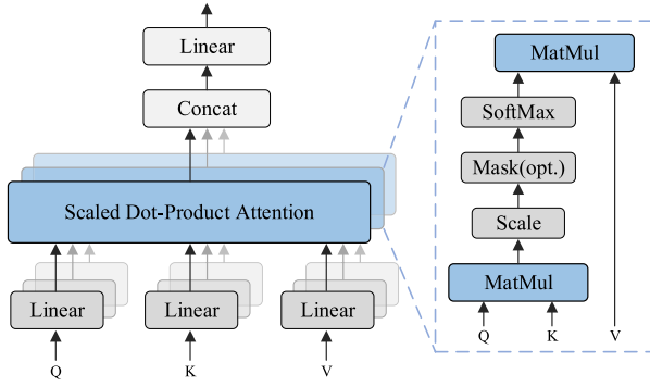
Fig. 1. Architecture of MHSA.
