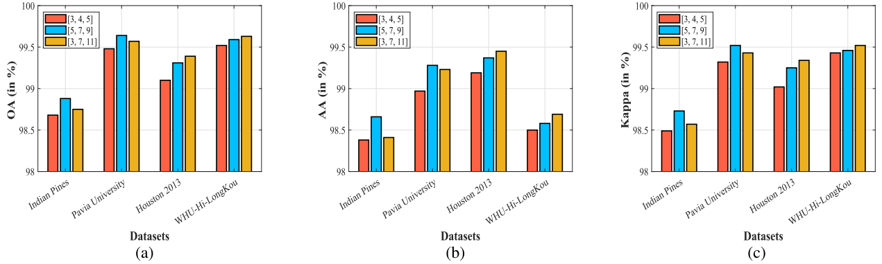
Fig. 12. Sensitivity analysis for the proposed method with different scales in terms of (a) OA, (b) AA, and (c) Kappa.
