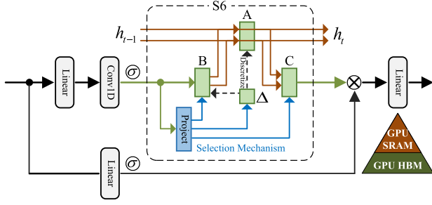
Fig. 2. Architecture of the Mamba block.
