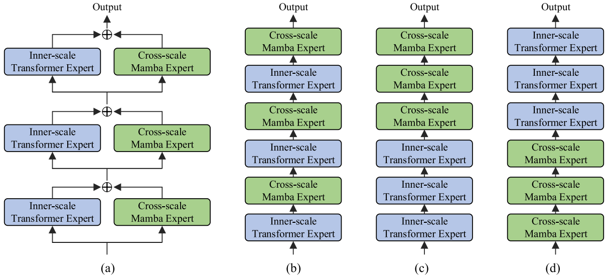
Fig. 4. Hybrid structures for HSI-MFormer. (a) Parallel structure. (b) Interval structure. (c) Serial structure v1. (d) Serial structure v2.
